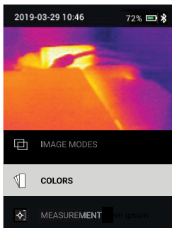
Figure 11.9 Select COLOURS from the IMAGE ADJUSTMENTS menu.
